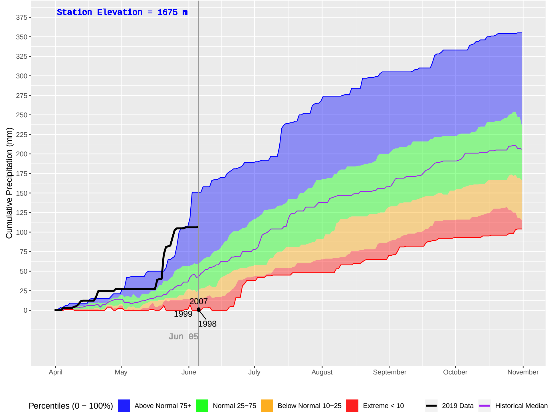
GASPARD (222) : Historical (1992–2018), Current (2019) Daily Cumulative Precipitation
