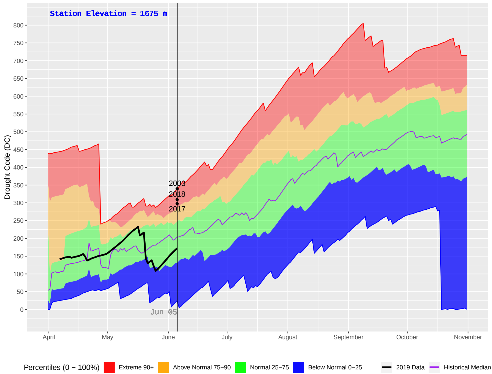
GASPARD (222) : Historical (1992–2018) and Current (2019) Daily Drought Code (DC)
