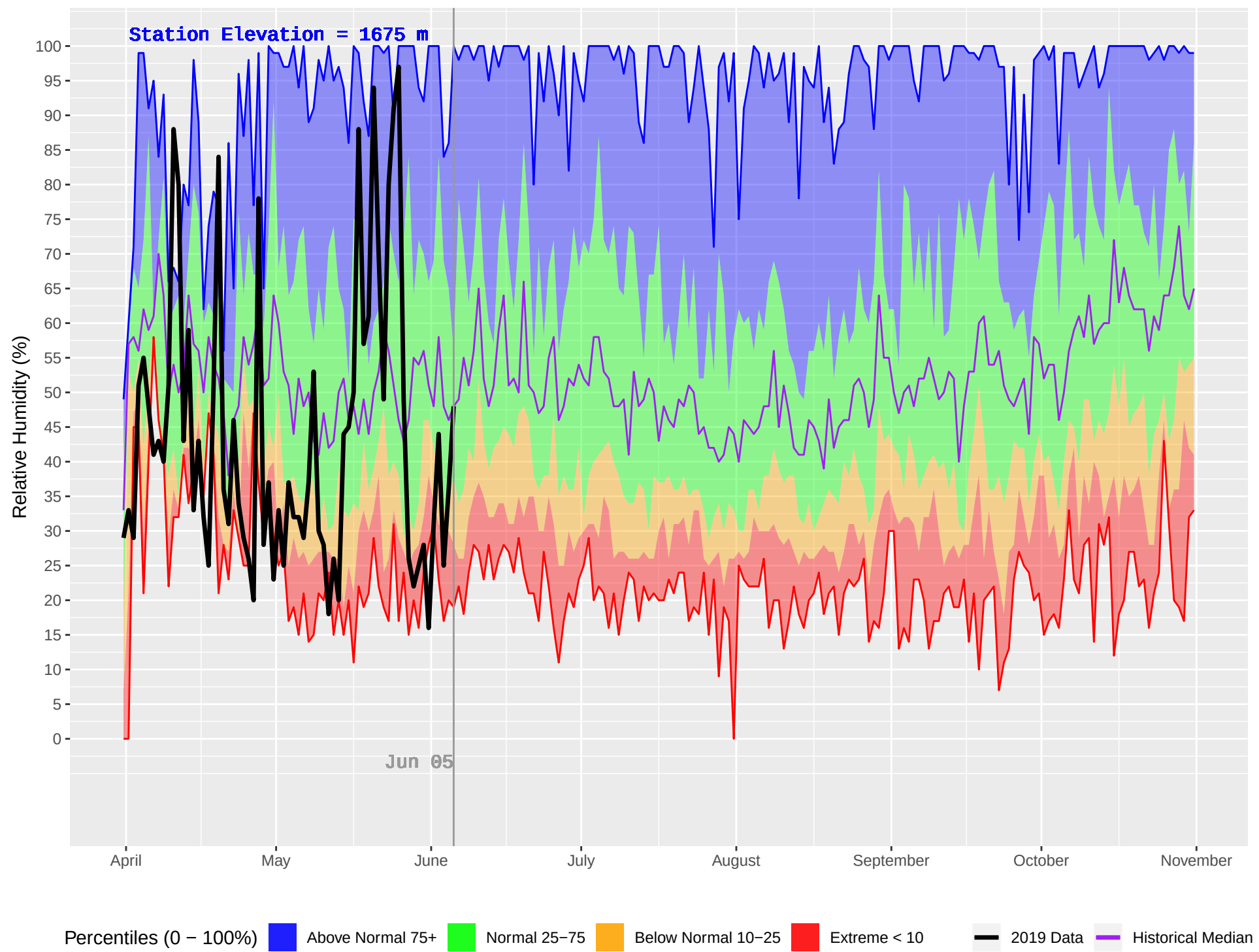
GASPARD (222) : Historical (1992–2018) and Current (2019) Daily Relative Humidity
