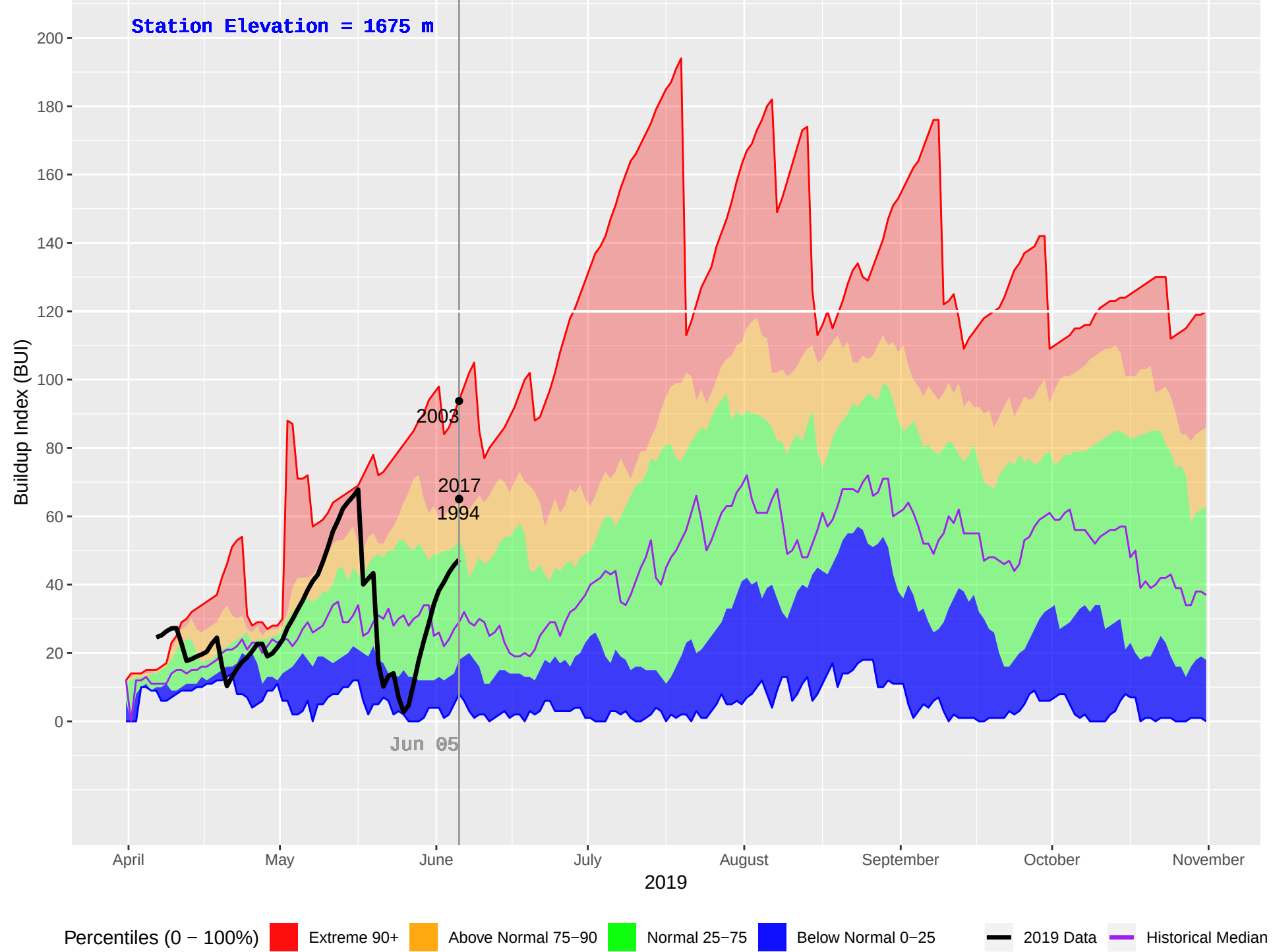
GASPARD (222) : Historical (1992–2018), Current (2019) Daily Buildup Index (BUI)
