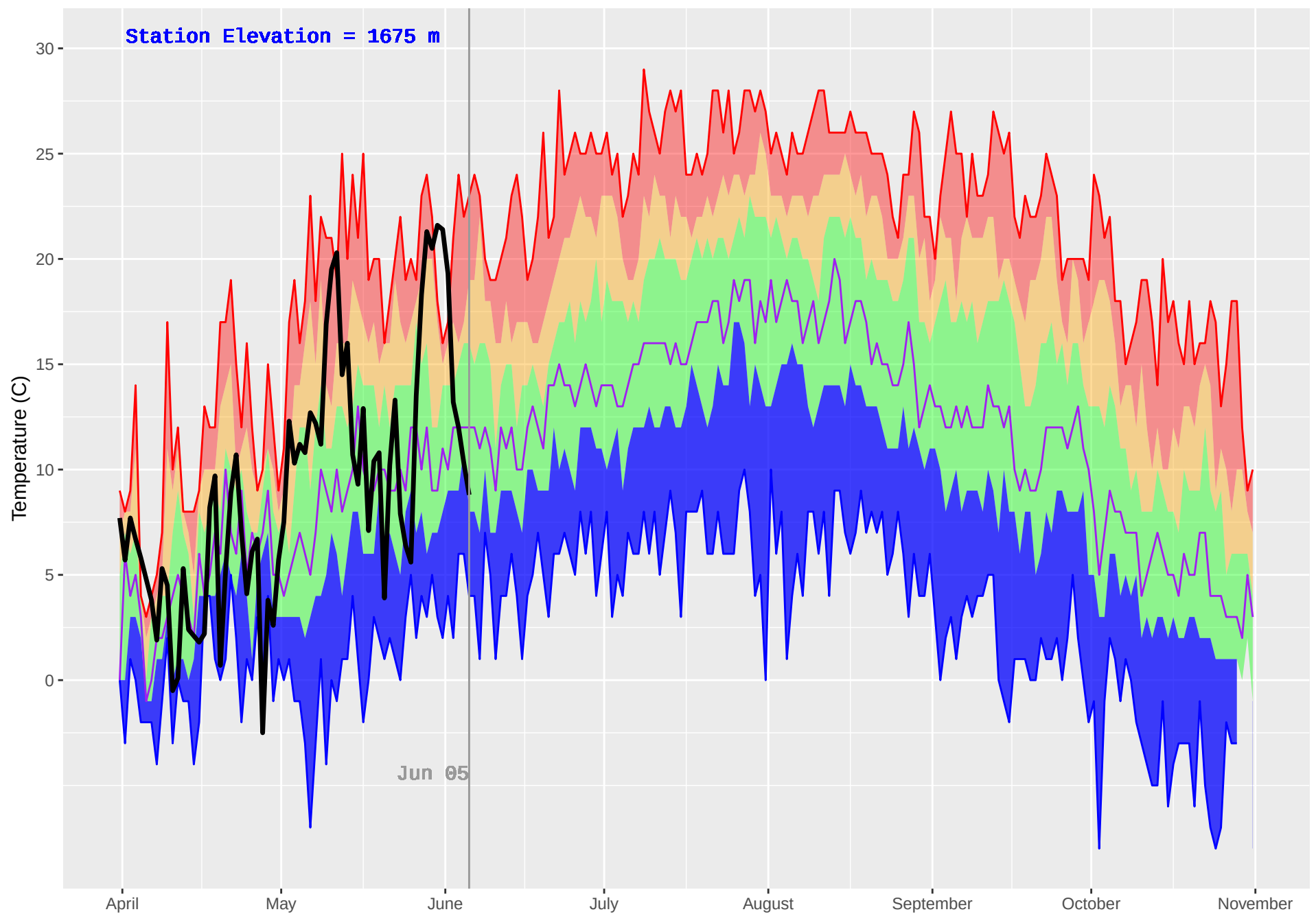
GASPARD (222) : Historical (1992–2018) and Current (2019) Daily Temperature
