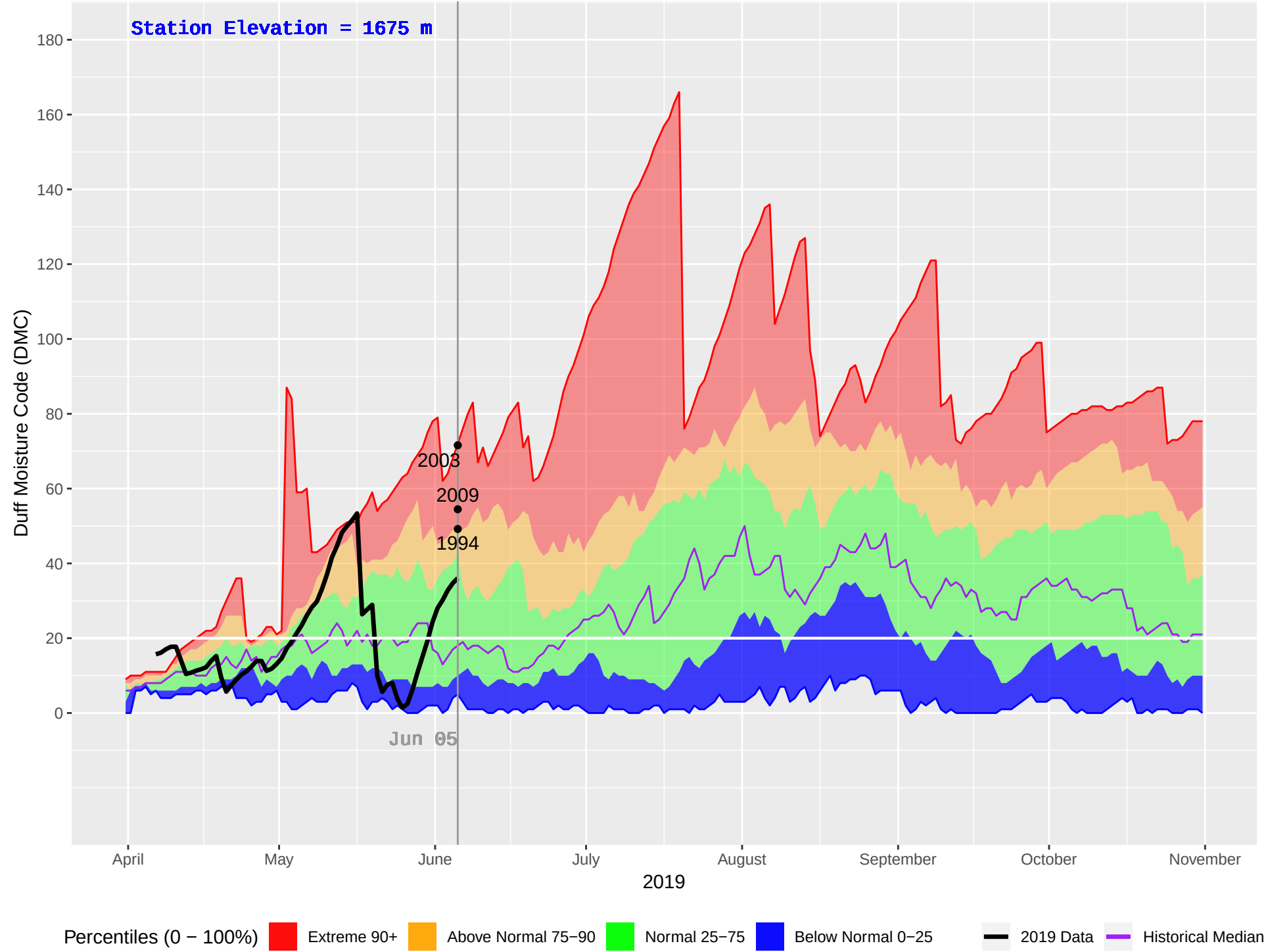
GASPARD (222) : Historical (1992–2018), Current (2019) Daily Duff Moisture Code (DMC)
