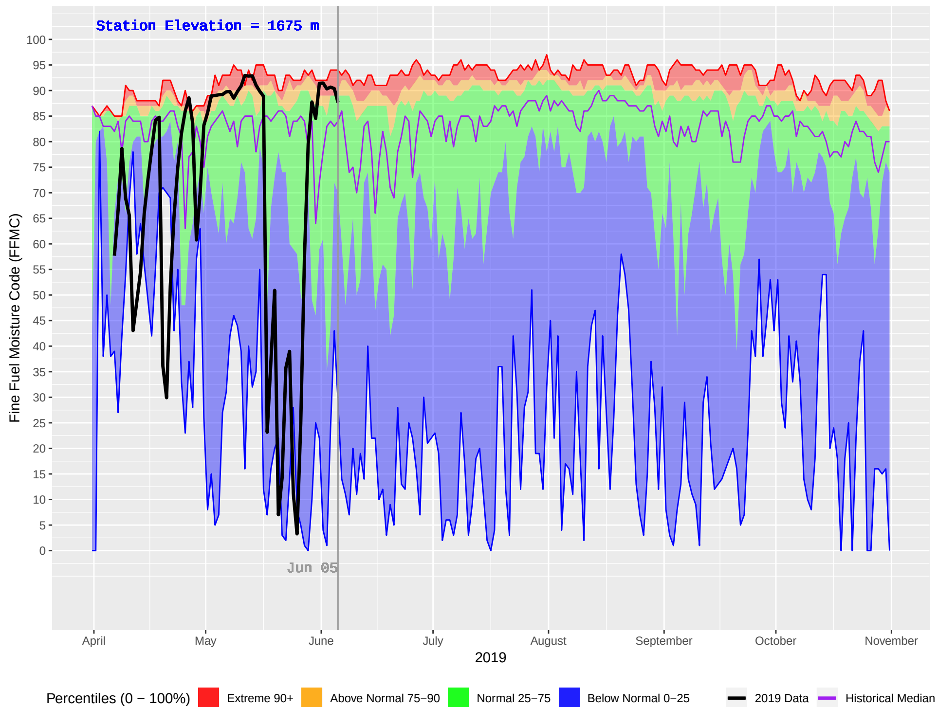
GASPARD (222) : Historical (1992–2018) and Current (2019) Daily Fine Fuel Moisture Code (FFMC)
